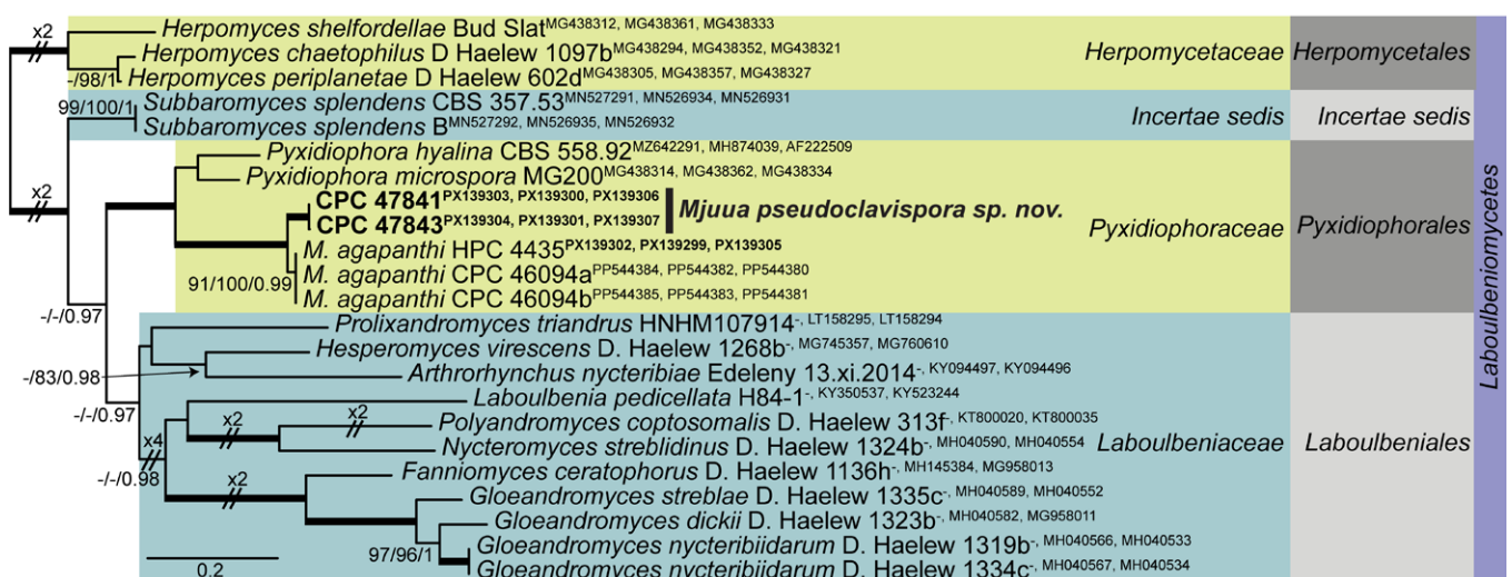
Fig. 37. Mjuua pseudoclavispora . Most likely phylogram obtained from the maximum likelihood analysis with IQ-TREE v. 2.4.0 (Kalyaanamoorthy et al. 2017, Minh et al. 2020, Mo et al. 2023) of the Laboulbeniomycetes ITS-LSU-SSU nucleotide alignment. Bootstrap support values (BS) > 74 % from 1000 ultrafast bootstrap replicates are shown at the nodes, followed by BS from 1000 non-parametric replicates on raxmlGUI 2.0 (Stamatakis (2014), Edler et al. (2021)), and bayesian posterior probability values > 0.84 obtained using MrBayes v. 3.2.7a (Ronquist et al. 2012). Thickened branches indicate full support (BS = 100 and PP = 1). Culture collection or specimen voucher numbers and GenBank accession numbers (superscript ITS, LSU and SSU, respectively) are indicated for all species. The tree was rooted to the Herpomycetaceae ( Herpomyces chaetophilus D Haelew 1097b, H. periplanetae D Haelew 602d and H. shelfordellae Bud Slat) and the novelty described here is indicated in bold font. Alignment statistics: 23 strains including the outgroup; 2654 characters including alignment gaps analysed: 922 parsimony-informative, 1414 constant sites. The best-fit models identified in IQ-TREE using the TESTNEW option and MrModelTest (Posada & Crandall 1998) were, respectively: ITS (1727–2654): HKY+F+I+G4, GTR+I+G; LSU (1–936): TIM3+F+I+G4, GTR+I+G; SSU (937–1726): TIM3+F+G4, GTR+I+G. The scale bar shows the expected number of nucleotide substitutions per site. The alignment and tree were deposited at figshare.com (doi: 10.6084/m9.figshare.31353595).
