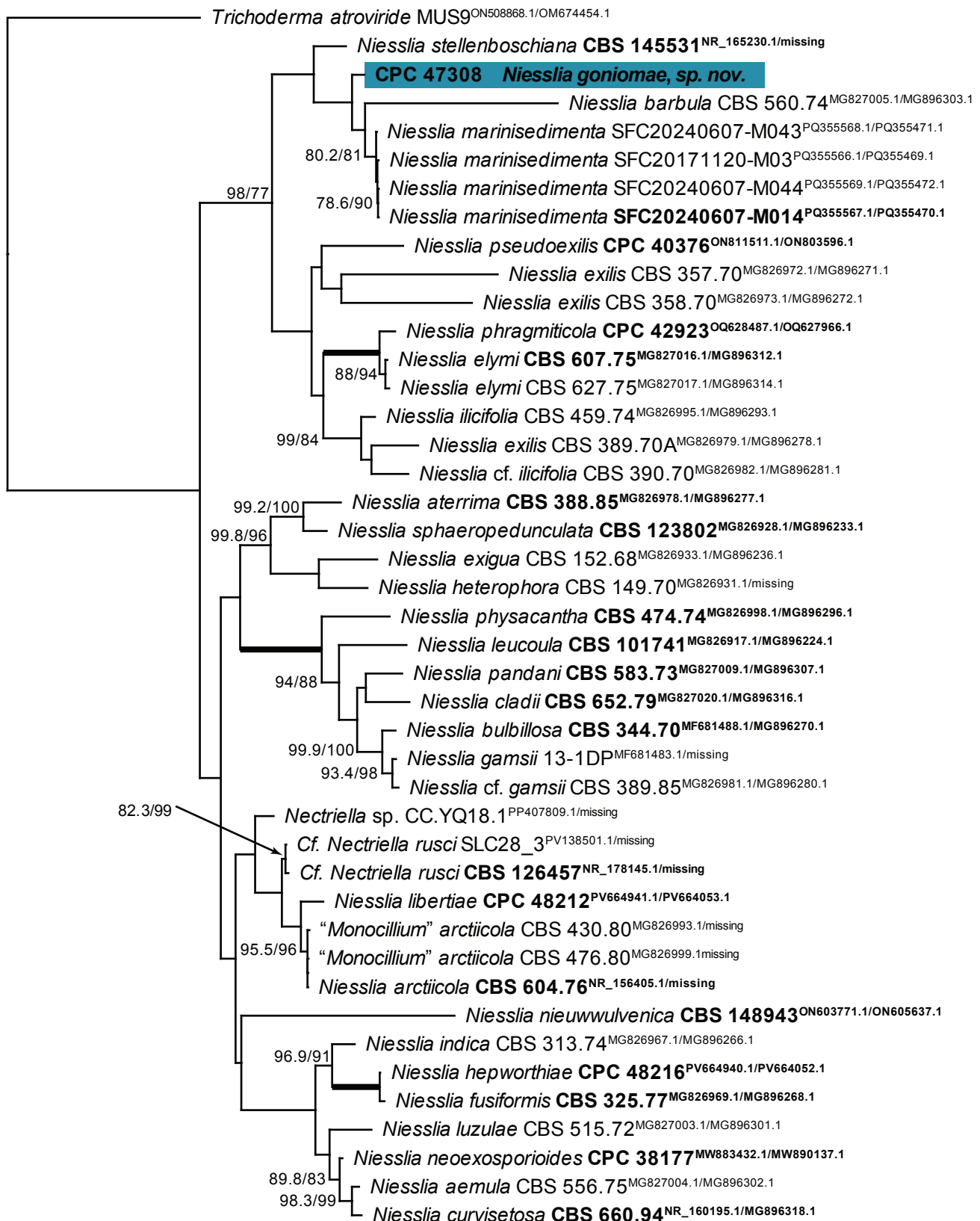
Fig. 39. Most likely phylogram obtained from the maximum likelihood analysis with IQ-TREE v. 2.4.0 (Kalyaanamoorthy et al. 2017, Minh et al. 2020, Mo et al. 2023) of the Niesslia ITS- tub2 nucleotide alignment. Bootstrap support values from 1000 non-parametric bootstrap replicates are shown at the nodes (> 74 % are shown), preceded by the SH-aLRT test value (only shown if the node has > 74 % bootstrap support). Thickened branches represent a SH-aLRT test value of 100 and a bootstrap support value of 100 %. Culture collection or specimen voucher numbers and GenBank accession numbers (superscript) are indicated for all species. Sequences from material with a type status are indicated in bold font. The tree was rooted to Trichoderma atroviride (MUS9; GenBank ON508868.1/OM674454.1) and the novelty described here is highlighted with a coloured block and bold font. Alignment statistics: 43 strains including the outgroup; 1131 characters including alignment gaps analysed: 700 distinct patterns, 453 parsimony-informative, 130 singleton sites, 548 constant sites. The best-fit models identified in IQ-TREE using the TESTNEW option were: ITS (1–651): TIM2+F+I+G4; tub2 (652–1131): TIM3+F+I+G4. The scale bar shows the expected number of nucleotide substitutions per site. The alignment and tree were deposited at figshare.com (doi: 10.6084/m9.figshare.31353595).
