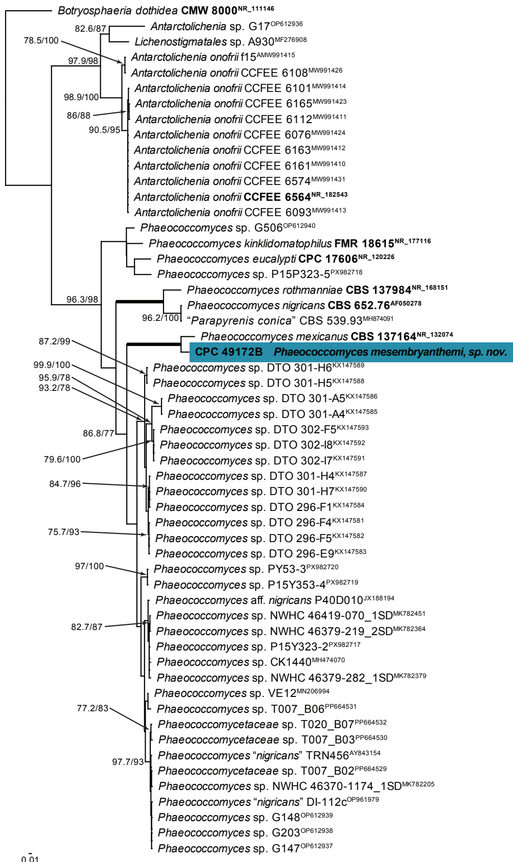
Fig. 49. Most likely phylogram obtained from the maximum likelihood analysis with IQ-TREE v. 2.4.0 (Kalyaanamoorthy et al. 2017, Minh et al. 2020, Mo et al. 2023) of the Phaeococcomyces ITS nucleotide alignment. Bootstrap support values from 1000 non-parametric bootstrap replicates are shown at the nodes (> 74 % are shown), preceded by the SH-aLRT test value (only shown if the node has > 74 % bootstrap support). Thickened branches represent a SH-aLRT test value of 100 and a bootstrap support value of 100 %. Culture collection or specimen voucher numbers and GenBank accession numbers (superscript) are indicated for all species. Sequences from material with a type status are indicated in bold font. The tree was rooted to Botryosphaeria dothidea (CMW 8000; GenBank NR_111146) and the novelty described here is highlighted with a coloured block and bold font. Alignment statistics: 55 strains including the outgroup; 581 characters including alignment gaps analysed: 315 distinct patterns, 205 parsimony-informative, 50 singleton sites, 326 constant sites. The best-fit model identified for the entire alignment in IQ-TREE using the TESTNEW option was: TIM2e+R3. The scale bar shows the expected number of nucleotide substitutions per site. The alignment and tree were deposited at figshare.com (doi: 10.6084/m9.figshare.31353595).
